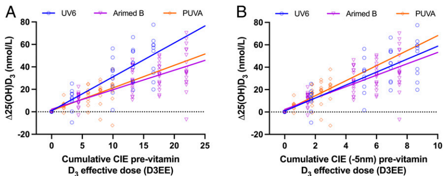
Fig. 6. FB linear regressions (with no baseline correction) for \Delta 25(\text{OH})\text{D}_3 versus UVR dose weighted with CIE pre-vitamin D action spectrum with (A) no shift or (B) 5-nm blue shift. Regression parameters, not forced through zero, for (A) no shift: UV6 y = 3.0x + 0.86 , Arimed B y = 1.7x + 2.26 , and PUVA y = 2.0x + 1.1 for (B) 5-nm shift: UV6 y = 5.8x + 0.86 , Arimed B y = 5.1x + 2.26 , and PUVA y = 6.7x + 1.12 . All R^2 and P values for a given spectrum as for Fig. 4B. The common model including baseline correction: 25(\text{OH})\text{D} (in nmol/L) = 4.05[2.04] ( P = 0.049 ) + 0.95[0.05] ( P = 0.32 compared to 1) \times pre-25(OH)D - 0.059[0.012] ( P = 1.54 \times 10^{-6} ) \times pre-25(OH)D \times D3EE + 7.35[0.46] ( P = 6.95 \times 10^{-37} ) \times D3EE, [SD]. 1 D3EE = 100J/m 2 weighted by the CIE pre-vitamin D 3 action spectrum with or without 5-nm blue shift.
