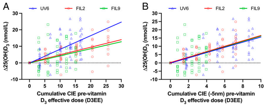
Fig. 5. PB linear regressions (with no baseline correction) for \Delta 25(\text{OH})\text{D}_3 versus UVR dose weighted with CIE pre-vitamin D action spectrum with (A) no shift or (B) with 5-nm blue shift. Regression parameters, not forced through zero, for (A) no shift: UV6 y = 0.8x - 0.1 , filter 2 y = 0.5x + 0.26 , filter 9 y = 0.4x - 0.04 and for (B) 5-nm shift: UV6 y = 1.6x - 0.09 , filter 2 y = 1.6x + 0.26 , filter 9 y = 1.6x - 0.04 . All R^2 and P values for a given spectrum as for Fig. 4A. The common model for 25(OH)D, including baseline correction: 25(\text{OH})\text{D} (in nmol/L) = -1.31[1.83] ( P = 0.47 ) + 1.04[0.051] ( P = 0.38 compared to 1) \times pre-25(OH)D - 0.033 [0.012] ( P = 0.0046 ) \times pre-25(OH)D \times D3EE + 2.64[0.41] ( P = 6.75 \times 10^{-10} ) \times D3EE, [SD]. 1 D3EE = 100J/m 2 weighted by the CIE pre-vitamin D 3 action spectrum with or without 5-nm blue shift.
